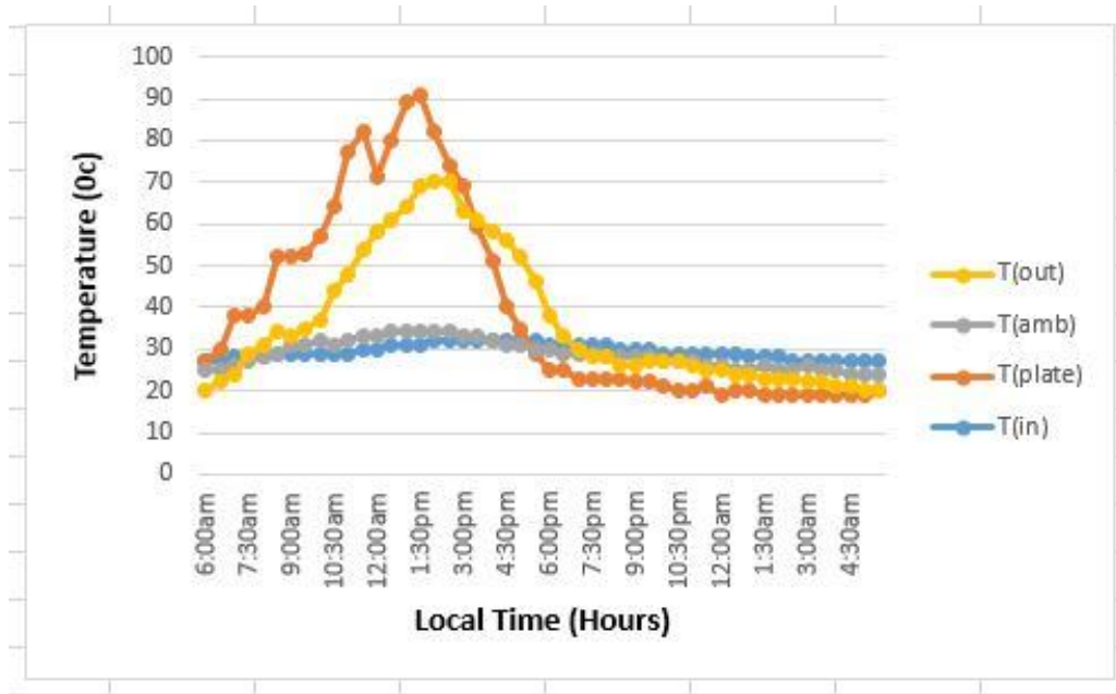
Fig. 6 Temperature variation with local time on a test day for Heating and Cooling Phases
