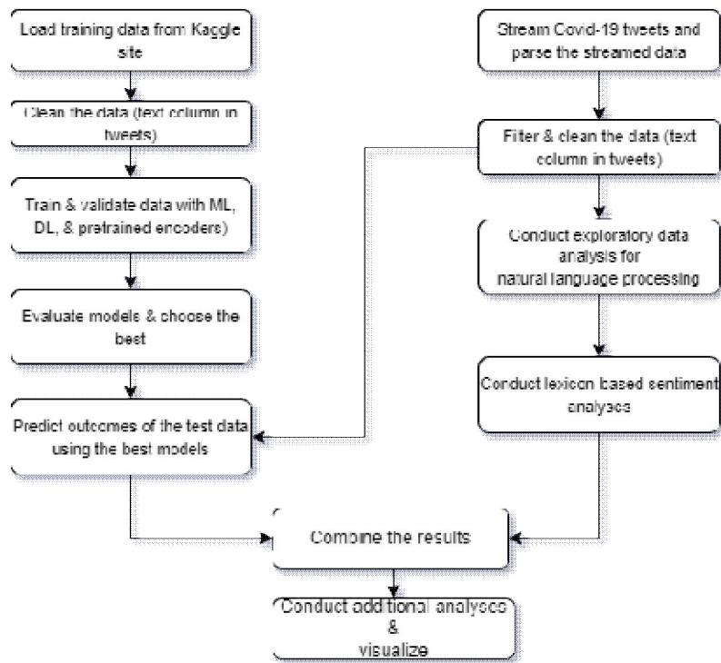
Figure 1. Processes of the Opinion Mining
