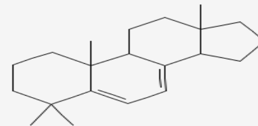
Structure of Androsta-5,7-diene, 4,4-dimethyl-
