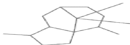
Structure of 1H-3a,7-Methanoazulene, octahydro-1,4,9,9-tetramethyl-
