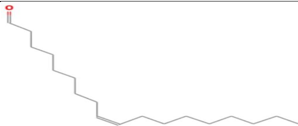
Structure of 9-Octadecenal, (Z)-
