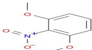
Structure of Benzene, 1,3-dimethoxy-2-nitro-
