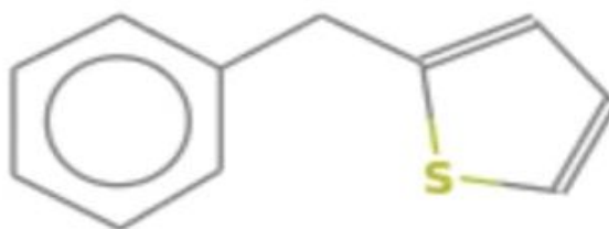
Structure of Thiophene, 2-(phenylmethyl)-
