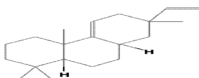
Structure of Isopimara-9(11),15-diene
