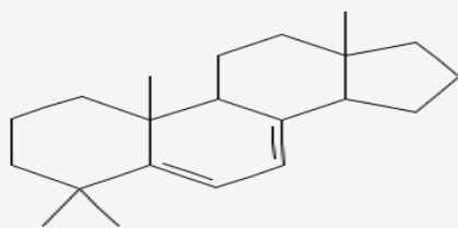
Structure of Androsta-5,7-diene, 4,4-dimethyl-
