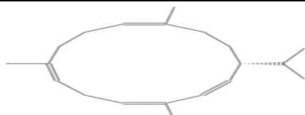
Structure of 1,3,6,10-Cyclotetradecatetraene, 3,7,11-trimethyl-14-(1-methylethyl)-, [S-(E,Z,E,E)]-
