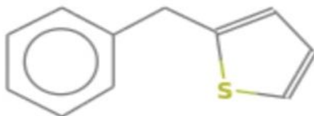
Structure of Thiophene, 2-(phenylmethyl)-
