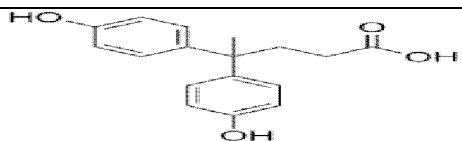
Structure of Diphenolic acid
