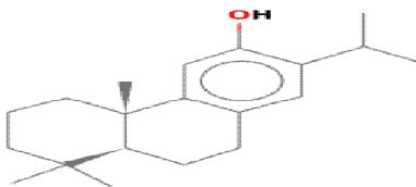
Structure of Ferruginol
