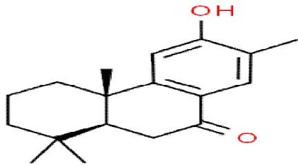
Structure of Nimbiol
