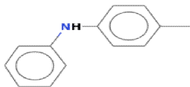
Structure of Benzenamine, 4-methyl-N-phenyl-
