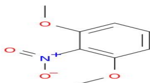
Structure of Benzene, 1,3-dimethoxy-2-nitro-
