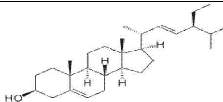
Structure of Stigmasterol
