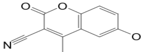
Structure of 2H-1-benzopyran-3-carbonitrile, 6-hydroxy-4-methyl-2-oxo-
