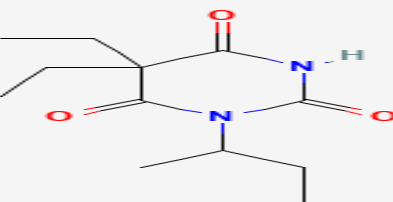
Structure of 2,4,6-(1H,3H,5H)-Pyrimidinetrione, 5,5-diethyl-1-(1-methylpropyl)-
