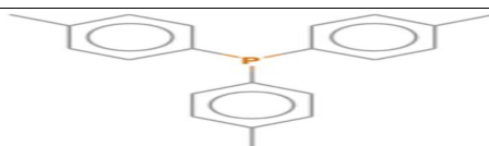
Structure of Phosphine, tris(4-methylphenyl)-
