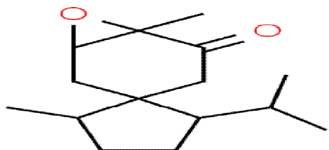
Structure of Spiro[4.5]decan-7-one, 1,8-dimethyl-8,9-epoxy-4-isopropyl-
