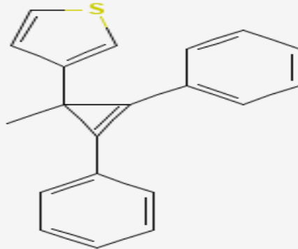
Structure of 3-Methyl-1,2-diphenyl-3-(3-thienyl)cyclopropene
