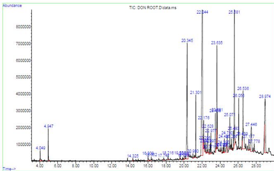
Figure 1: GC-MS Chromatogram of Azadirachta indica root
