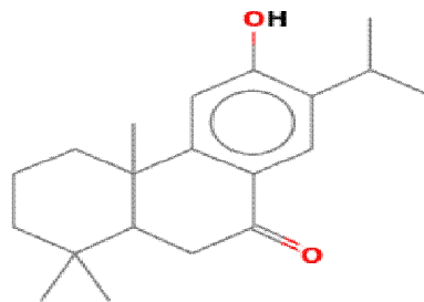
Structure of 9 (1H)-Phenanthrenone, 2,3,4,4a,10,10a-hexahydro-6-hydroxy-1,1,4a-trimethyl-7-(1-methylethyl)-, (4aS-trans)-
