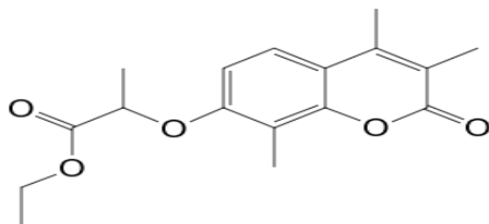
Structure of 2-(3,4,8-Trimethyl-2-oxo-2H-
