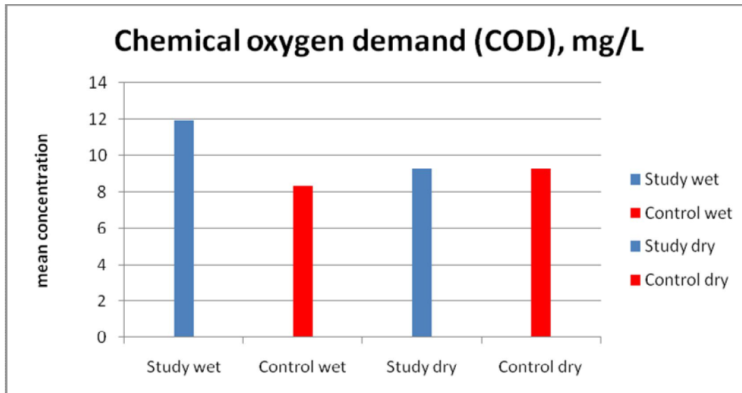
Figure 5: Mean concentration of chemical oxygen demand in study area
