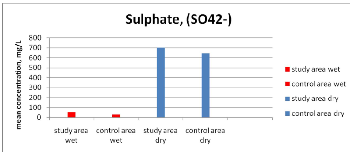
Figure 7: mean concentration of sulphate in the studyarea
