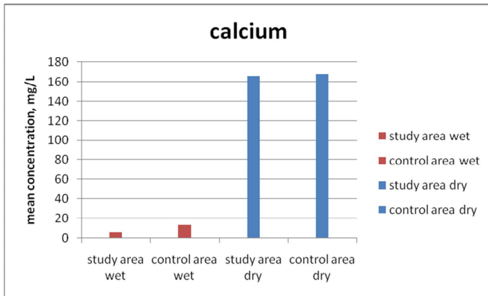
Figure 8: mean concentration of calcium from the study area
