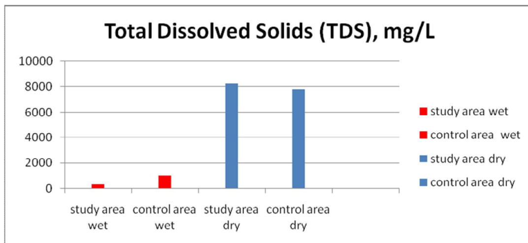
Figure 4: mean concentration of total dissolved solids from the study area.
