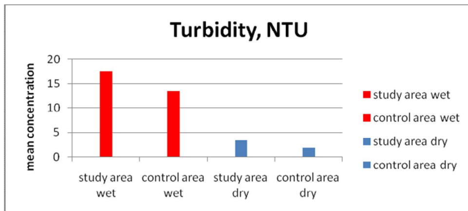
Figure 6. Mean concentration of turbidity from the study area
