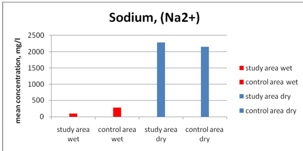
Figure 9: Mean concentration of sodium in study area
