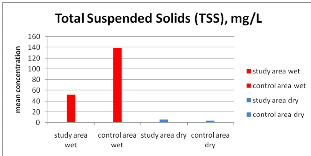
Figure 3: Mean concentration total suspended solids from the study area
