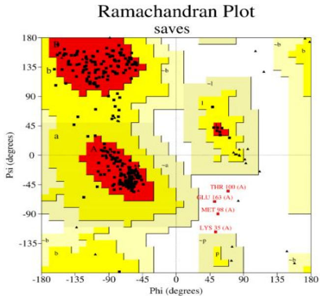
Fig. 5. Ramachandran plot showing the phi -psi torsion angles for all the residues of the chitinase protein: the distribution of amino acid residues to \beta -sheets (+psi, -phi), right-handed \alpha -helix (-psi, -phi) and left-handed \alpha -helix (+phi, +psi)
