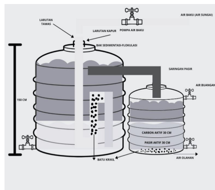
Figure 1. River Water Filtration Design
