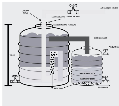
Figure 1. River Water Filtration Design
