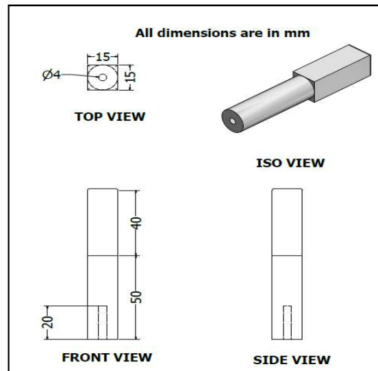
Fig. 4 Detailed drawing of metering shaft
