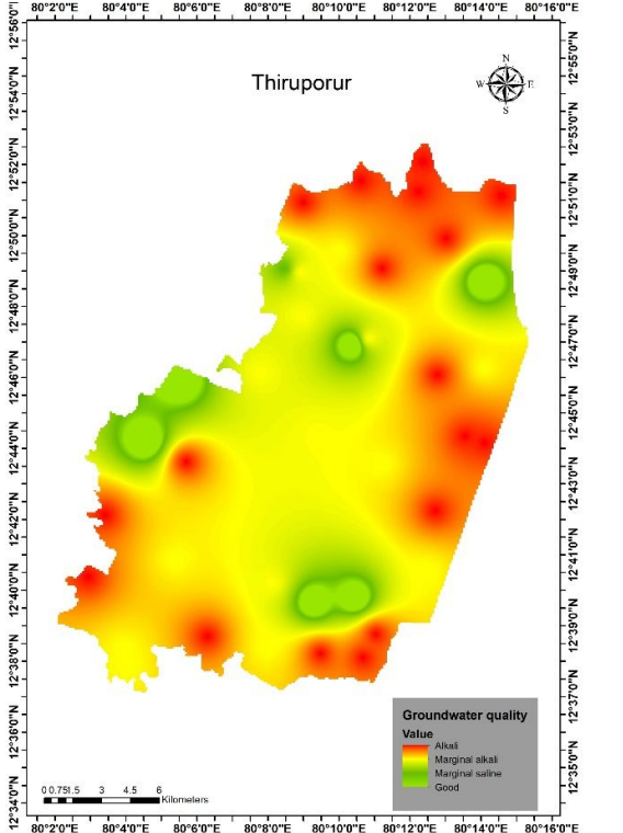
Fig.2. Spatial distribution of different quality parameters of groundwater in coastal blocks of Chengalpattu district
