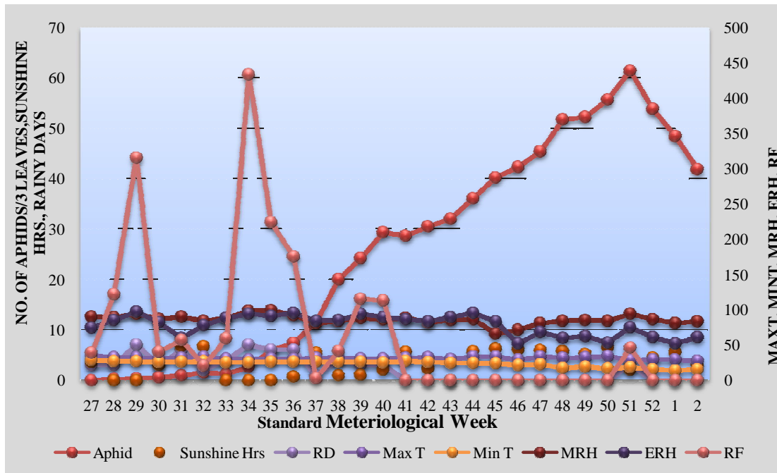
Fig. 2: Incidence of aphid, A. gossypiini in non- Bt cotton in relation to weather parameters
