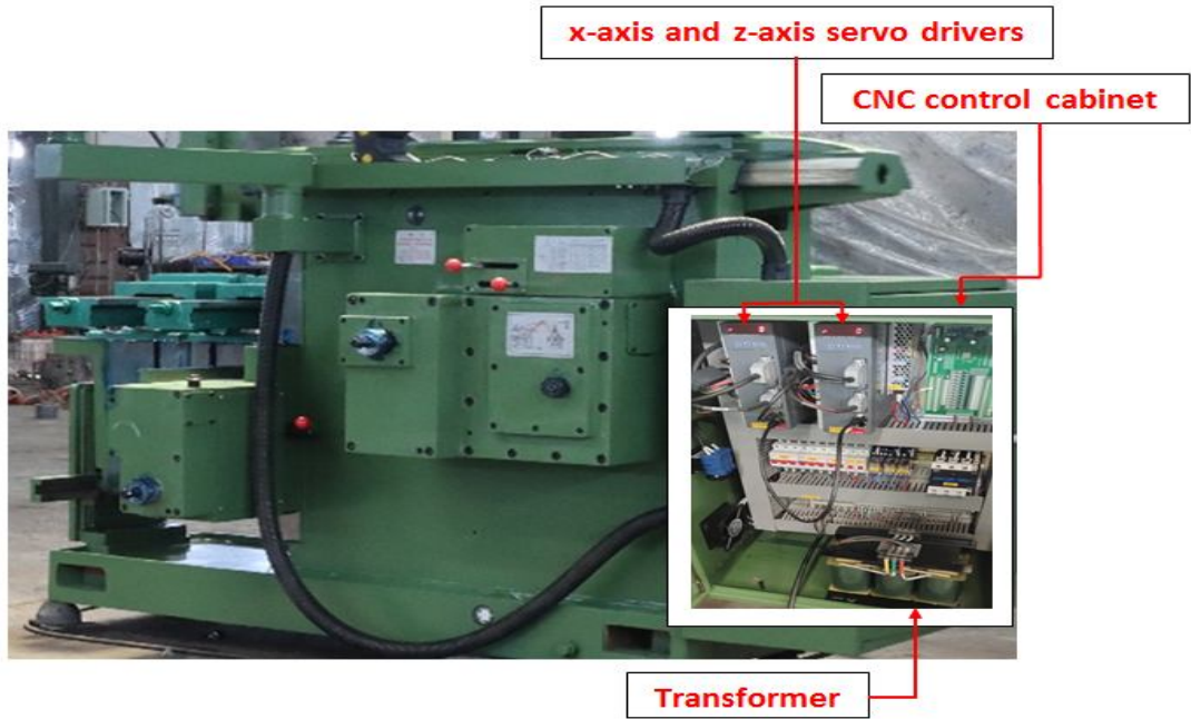
Fig. 2.CNC control cabinet
