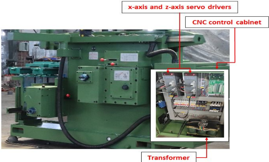
Fig. 2. CNC control cabinet
