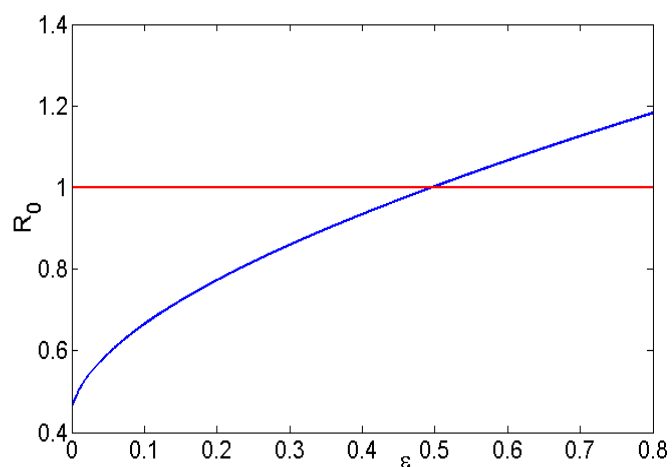
Figure 4: Effects of varying rate modifying factor for disease transmission modeled by parameter \epsilon on \mathcal{R}_0
