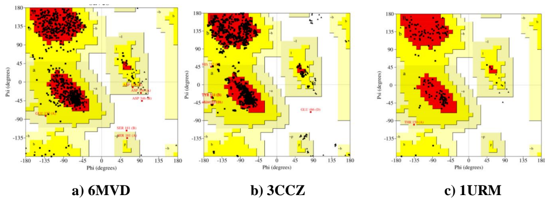
Figure 4: Ramachandran plot of protein 6MVD, 3CCZ and 1URM protein
