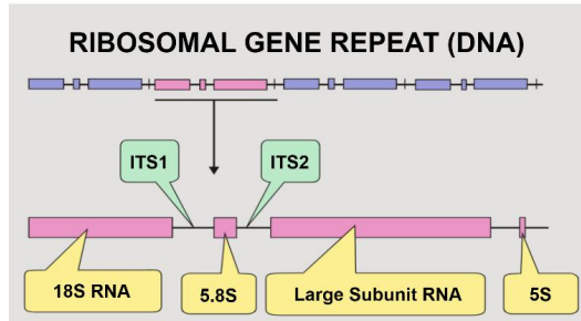
Figure 1. Ribosomal subunits and internal transcribed spacer region(18)
