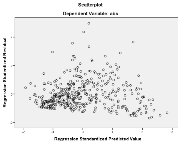
Figure 2 : Heteroscedasticity test
