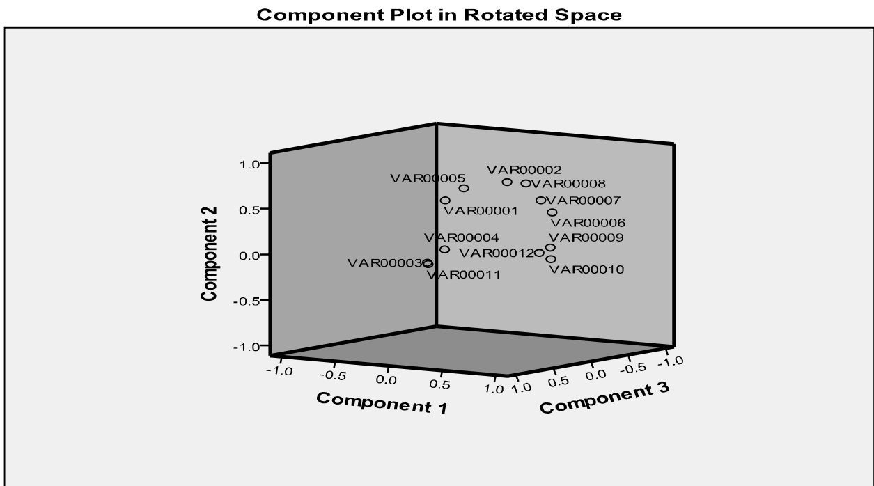
Fig 2 : Component Plot in Rotated Space
