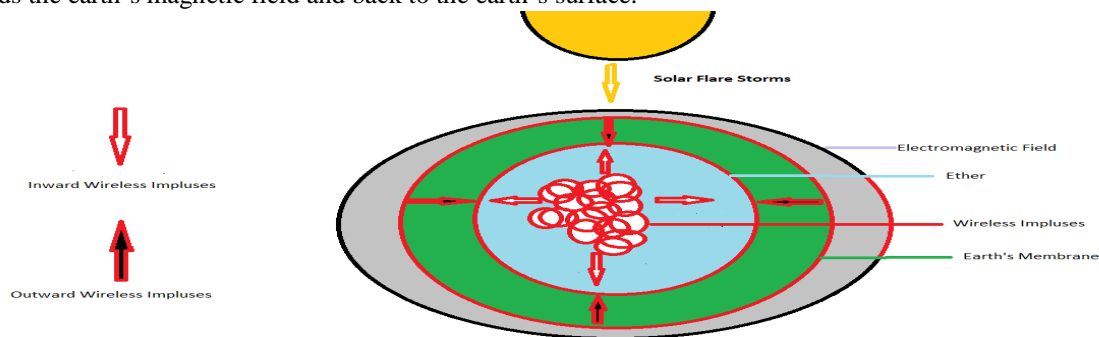
Figure A. The above pictorial illustrates the external stream of solar flare storms heading towards the earth's magnetic field, and the internal flow of wireless impulses through electromagnetic waves origination from the earth's surface towards earth's own magnetic field and back to the earth's surface.
