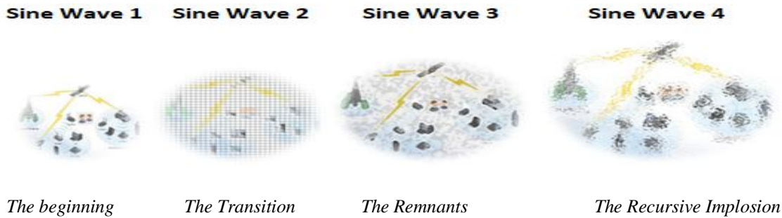
Figure H. The recursive sine wave delivers an escalation of electromagnetic wave pulses generated by nomadic wireless apparatuses into the remnants of an avalanche of heat. These massive (the beginning) and continuous electromagnetic waves (the transition) breed imperceptible heat that dissolves rapidly (the remnants) and is replaced simultaneously by another mass of electromagnetic activity (recursive implosion), hence, the byproduct of electromagnetic heat becoming a contributor to global warming.
