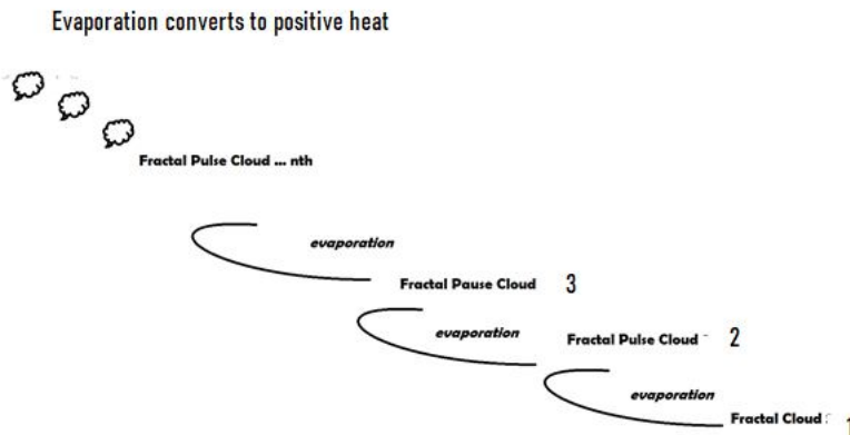
Figure I. The significance of fractal text pulse signals is that a singular electromagnetic mass that vaporizes rapidly is substituted immediately by another electromagnetic wave, and by another, until the bulk of the pulses are equal or of greater magnitude of the heat debris left by the mass of electromagnetic waves.
