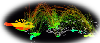
Figure E. The above global illustration of mobile phone (smart phone) interconnectivity provides a spectacular picture of electromagnetic waves generated by nomadic wireless instruments; an organic pulsing mass being distributed on the worldwide net. Should we consider electromagnetic waves any differently as a natural resource as we do of air, water, oil ...? What are the limits to growth for unleashing massive quantities of electromagnetic waves into the ecosphere?
