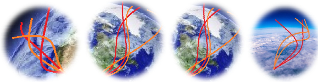
Figure B. The above illustration displays electromagnetic waves emanating from all geo-spaces on earth, and the rebounding of electromagnetic waves back to earth's surface.
