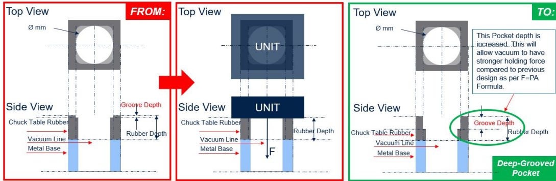
152 Fig. 5. Chuck Table Before and After
