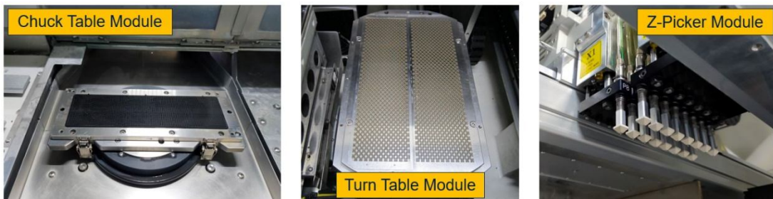
Note: Chuck table module, Turn Table module, and Z-Picker modules held the units using vacuum suction.
