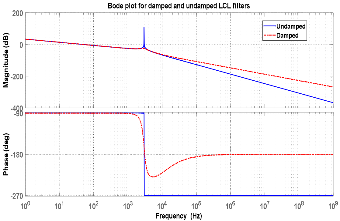
Figure 7: Bode plot for damped and undamped LCL filters
