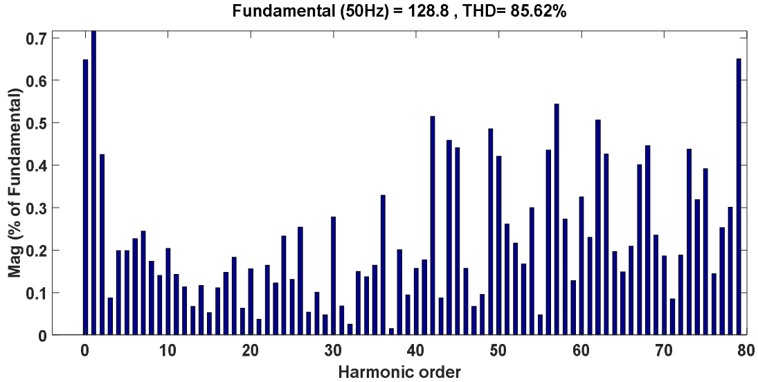
Figure 9: FFT analysis of the PV Inverter System
