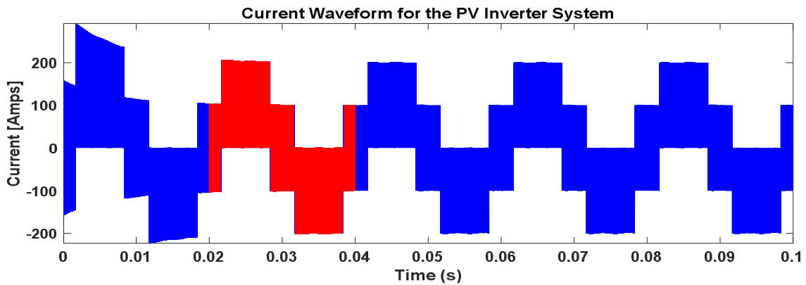
Figure 8: Current waveform of the PV Inverter System
