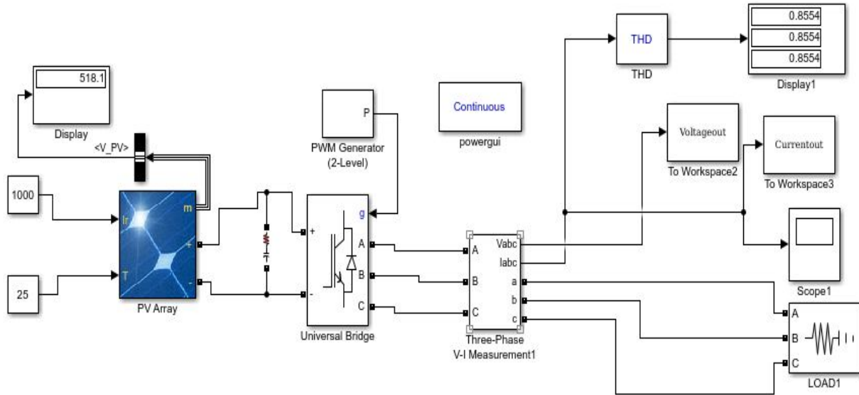
Figure 1: Simulink Model for Characterization of Harmonics in PV Inverter System
