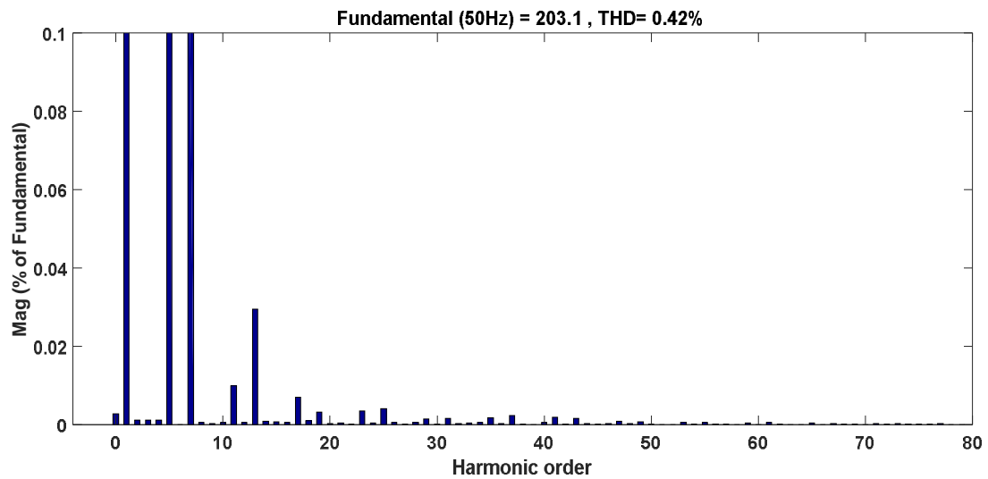
Figure 11: FFT analysis of the PV Inverter System with LCL filter
