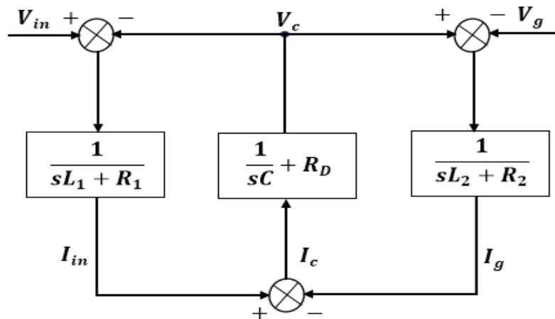
Figure 4: Block diagram of LCL Filter in S – Plane
