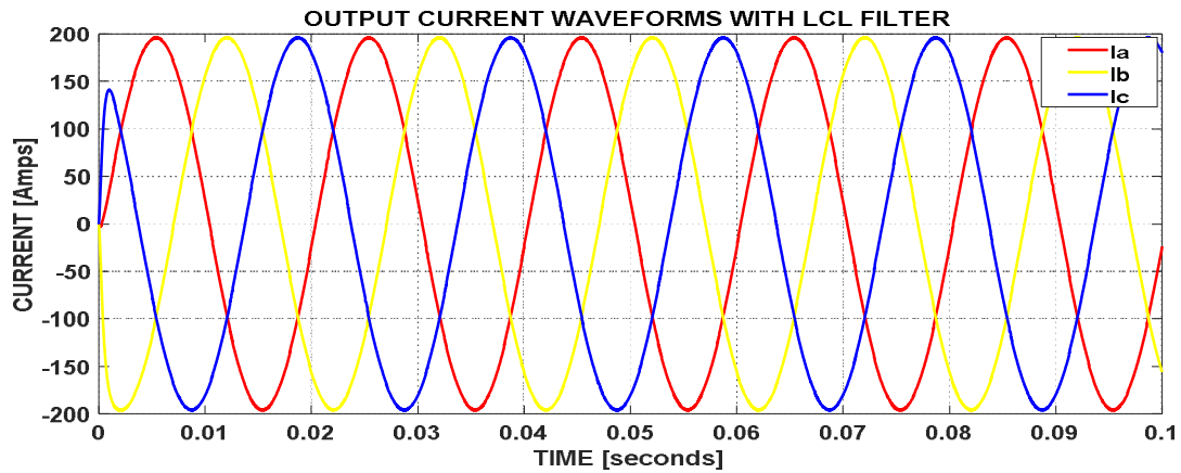
Figure 10: Three – phase Output Current Waveforms with LCL Filter
