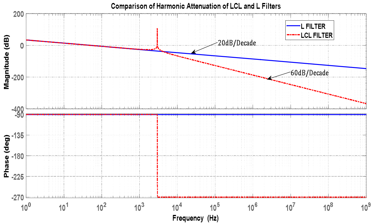
Figure 6: Comparison of Harmonic Attenuation of LCL and L Filters
