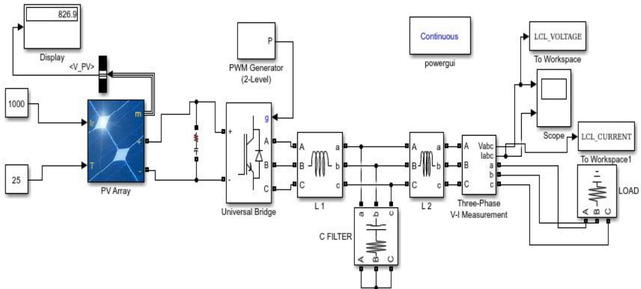
Figure 5: Simulink Model of the Inverter System with the LCL Filter
