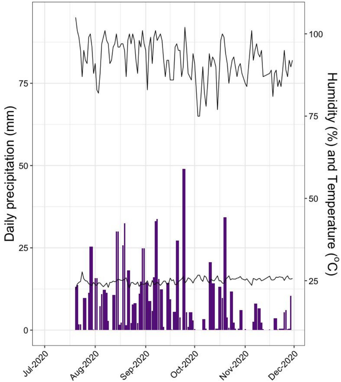
Figure 1. The total daily precipitation as bars (axis on left) and mean daily humidity-top (%) and mean daily temperature (°C) -bottom as lines (axis on right).
