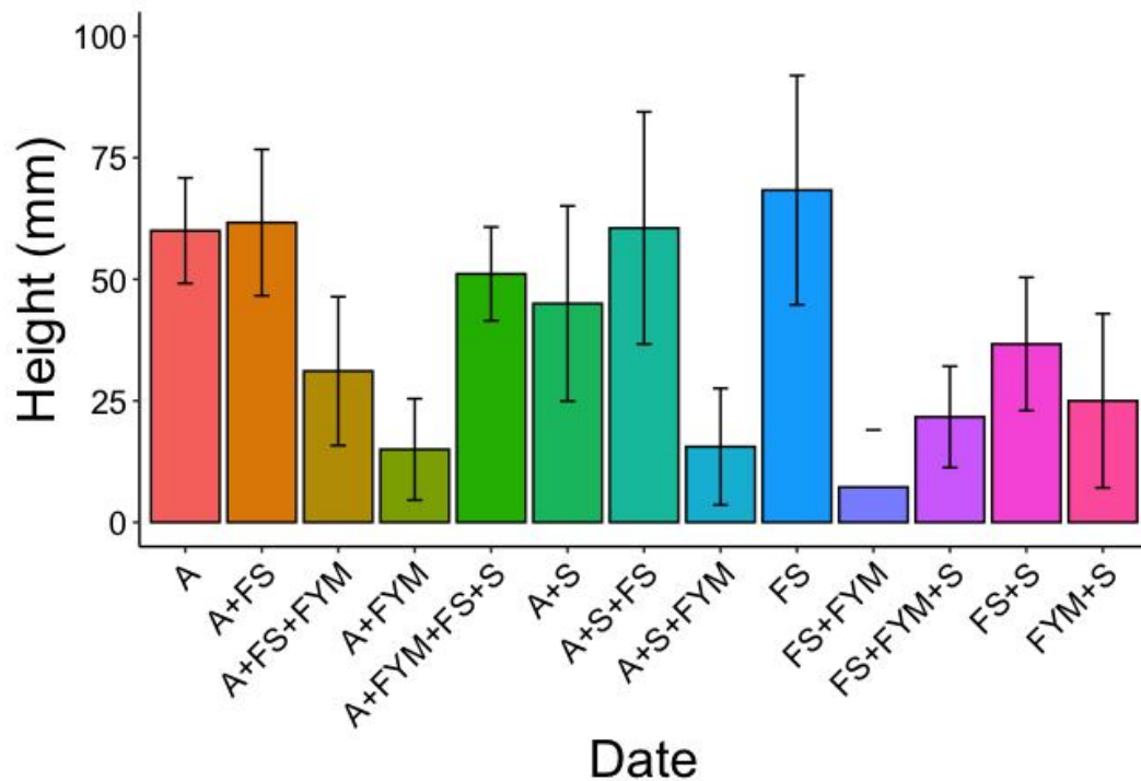
Figure 2 Mean final heights at month six for the seedlings of Cupressus lusitanica (a) and Grevillea robusta (b) for the various treatments of soil mixtures (A=Agricultural soil, FS =Forest soil, FYM = Farmyard Manure, S = Sand).
