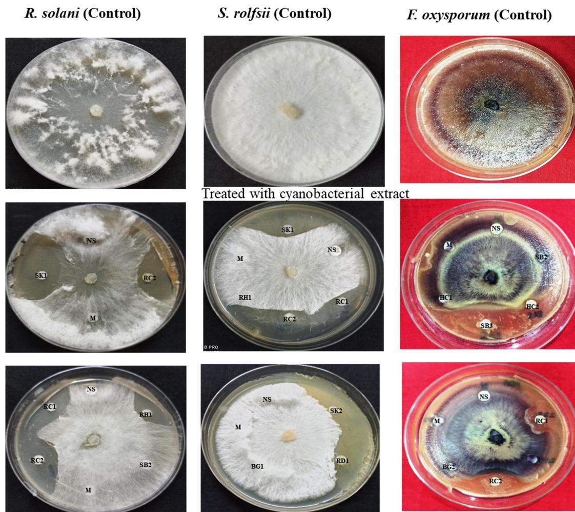
Figure 2. Antifungal activity of selected cyanobacteria against R. solani , S. rolfsii and F. oxysporum . SK1- Nostoc sp., RC2- Leptolyngbya sp, RC1- Leptolyngbya sp., RD1- Pseudoanabaena sp., SK2- Oscillatoria sp., Chroococcus sp SB3 Aphanothece sp., HC2 Nostoc sp. M-Methanol (Negative control), N-Nystatin (Positive control)
