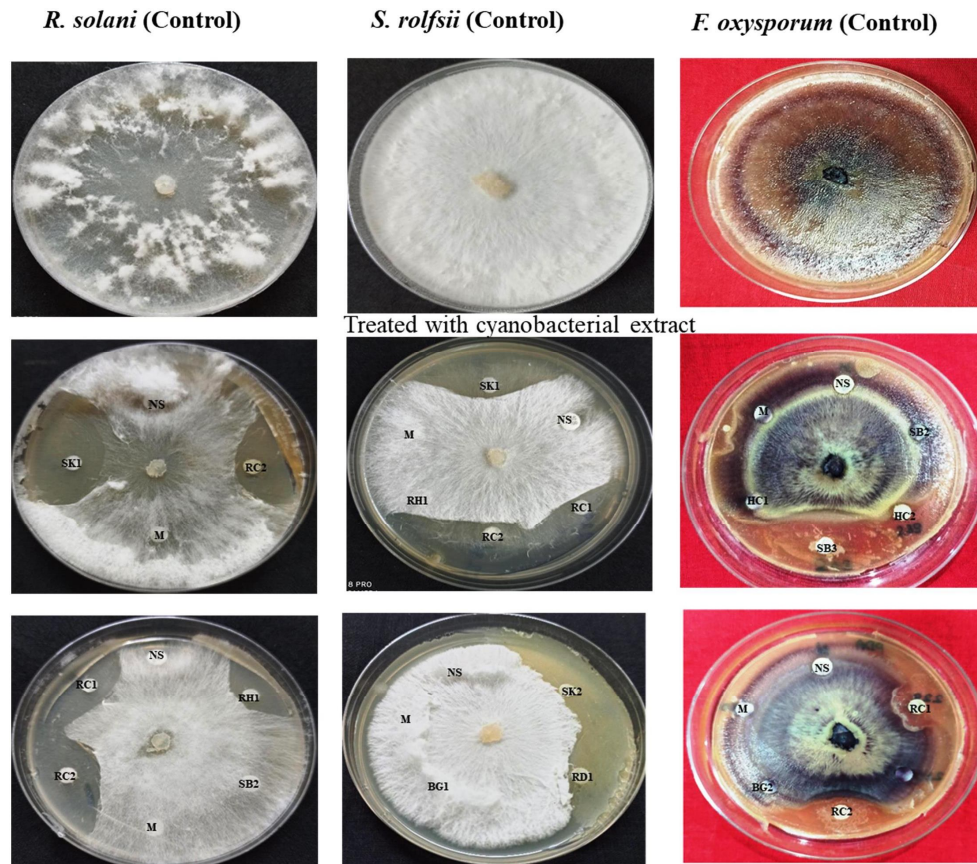
Figure 2. Antifungal activity of selected cyanobacteria against Rhizoctonia solani , Sclerotium rolfsii and Fusarium oxysporum . SK1- Nostoc sp., RC2- Leptolyngbya sp., RC1- Leptolyngbya sp., RD1- Pseudoanabaena sp., SK2- Oscillatoria sp., Chroococcus sp. SB3 Aphanothece sp., HC2 Nostoc sp. M-Methanol (Negative control), N-Nystatin (Positive control)
