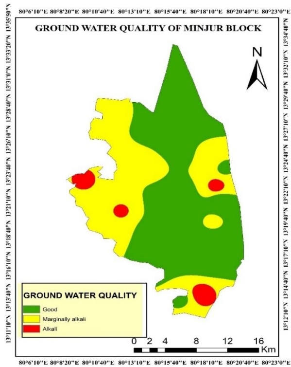
Figure 4: Spatial distribution of different quality parameters of groundwater in coastal blocks of Tiruvallur district:
