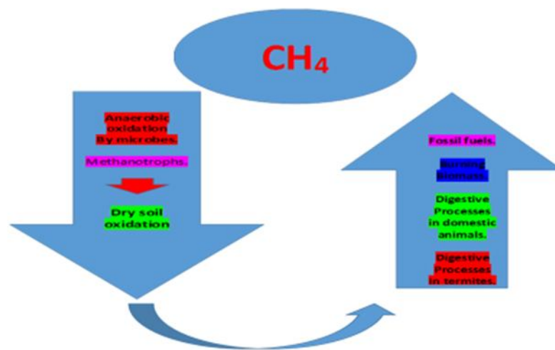
Figure 3: Methane cycle diagram.
