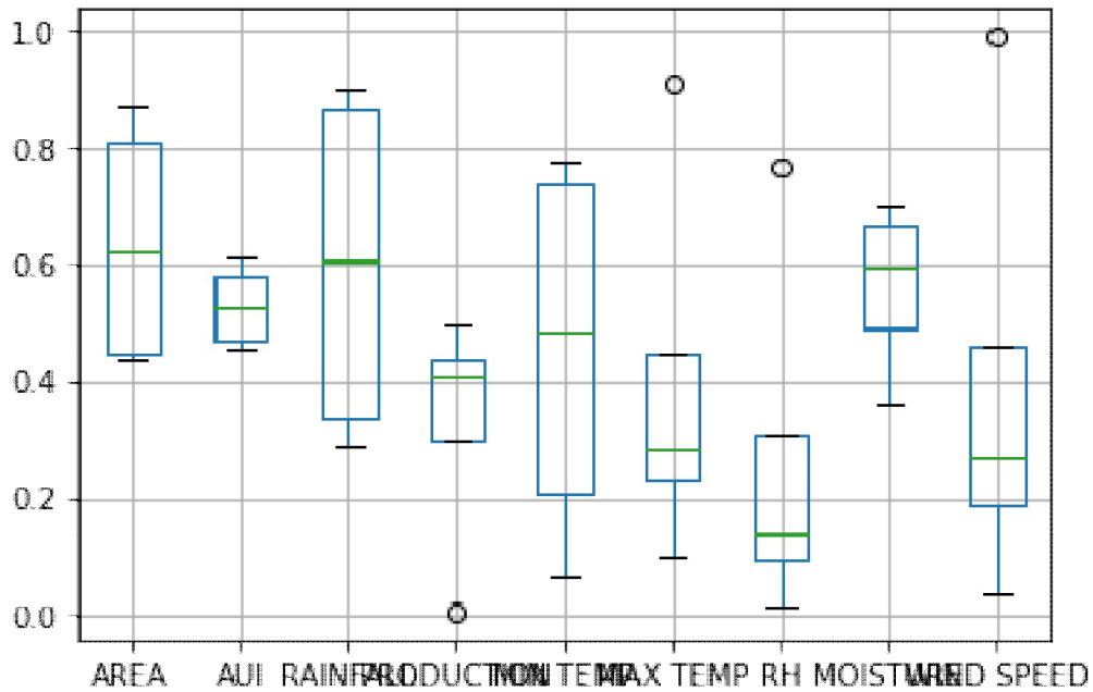
Figure 2 Box plot
