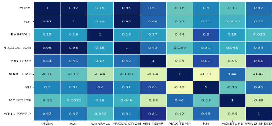
Figure.1 Correlation matrix
