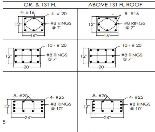
Fig 9(a): The columns' position, sizes, (b) Reinforcement details, in-ground, and floors
