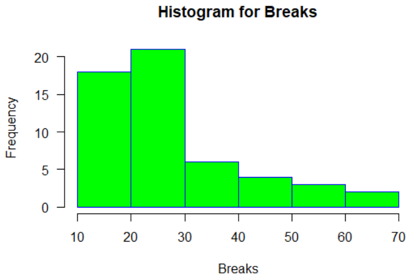
Fig.3. A histogram of the number of Breaks.
