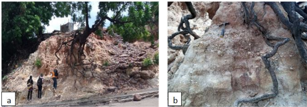
Figure 2: (a) Matrix supported Conglomerate facies of Lokoja formation at Robinson Street (N 07° 48' 46.8" E 06 ° 44' 40"). (b) Clasts embedded in the pebbly sandstone Conglomerate facies at Robinson Street (N07° 48' 46.8" E 06 ° 44' 40")
