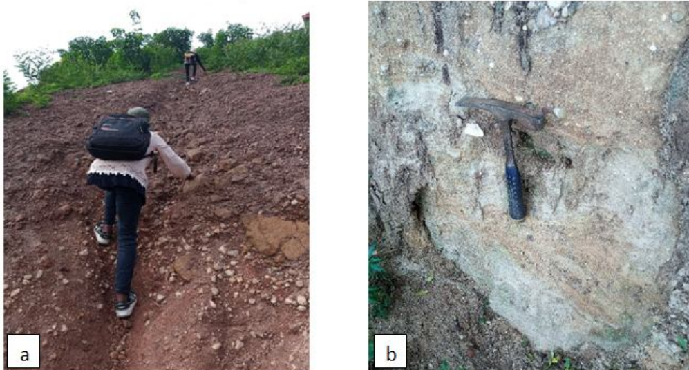
Figure 3: (a) Clasts supported fabric (paraconglomerate) exposed around in the Conglomerate facies in the hill at Kabawa (N 07 ° 49' 14.0" E 006 ° 44' 40"). (b)
