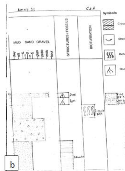
Figure 6: (a) Clasts embedded in massive, pebbly to coarse grained sandstone sub-facies at Opposite Cemetery, Kabawa (N 07 ° 49' 13" E 006 ° 44' 42.6"). (b) Lithologic section of the Lokoja Formation exposed at Ayoola Ajao Avenue, GRA.
