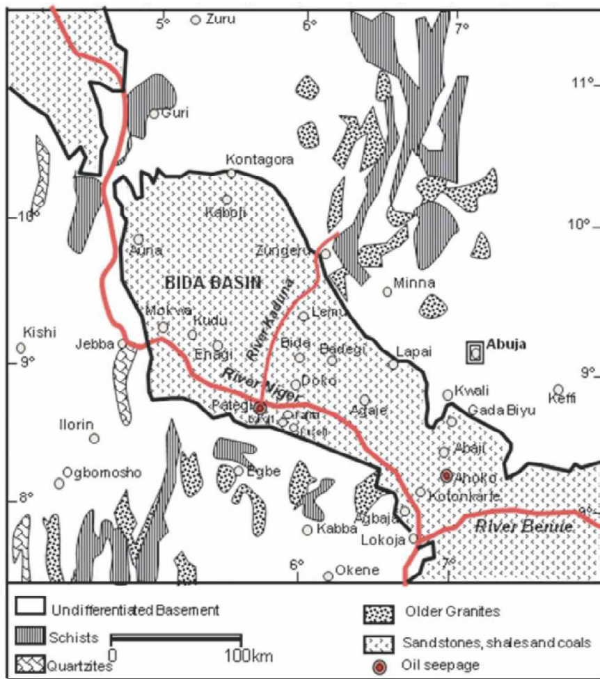
Figure.1.0: Geological and Location Map of Bida Basin and Environs (Obaje et al. , 2011)
