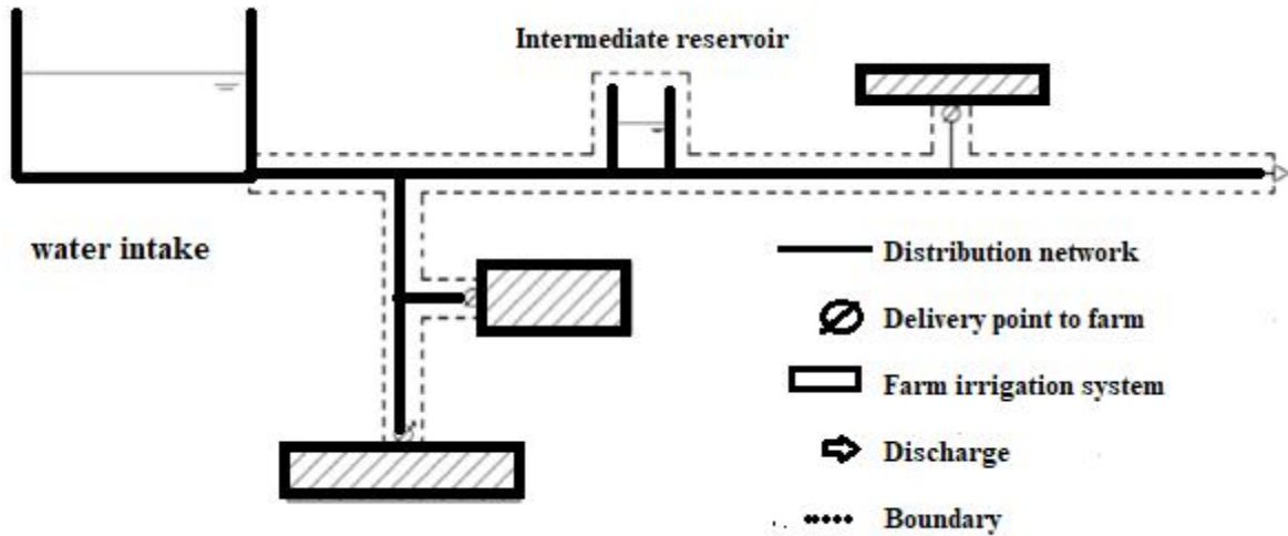
Fig 2. System boundary to consider for water balance calculation
