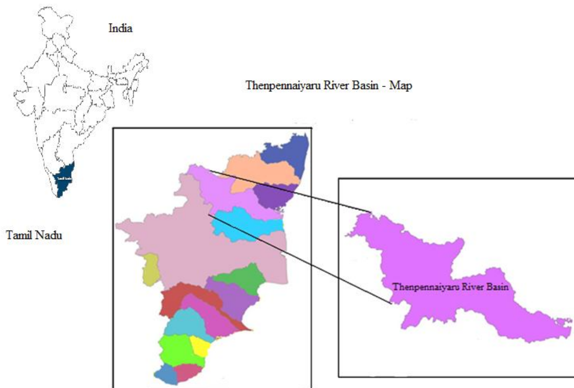
Fig 1. Study area Thenpennaiyar river basin of Tamil Nad
