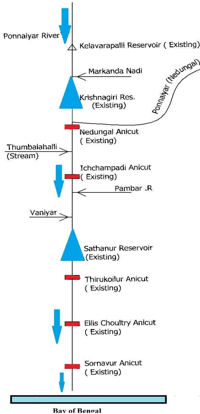
Fig 4. Schematic diagram of the Ponnaiyar river system with Major structures and link canal Source: Public Works Department Government of Tamil Nadu
