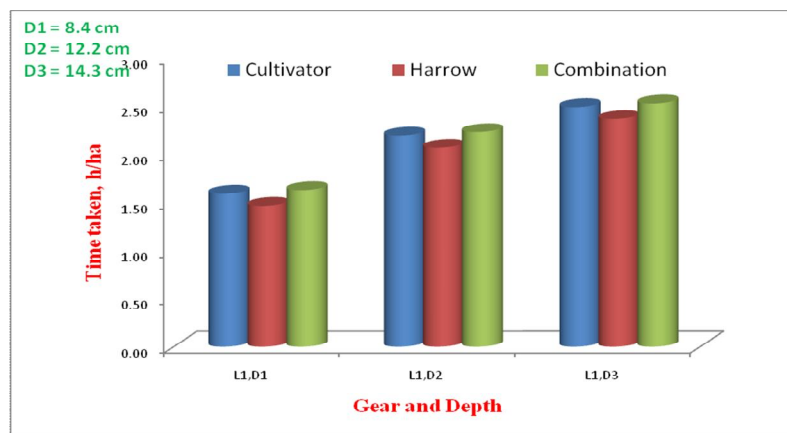
Fig.5 Comparison of time taken for field operations with different implements
