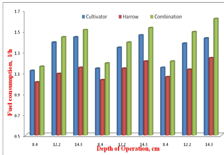
Fig.4 Effect of depth of operation on fuel consumption
