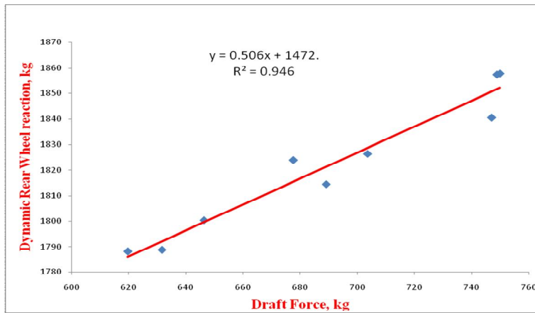
Fig. 6 Effect of draft force on dynamic rear wheel reaction of test tractor
