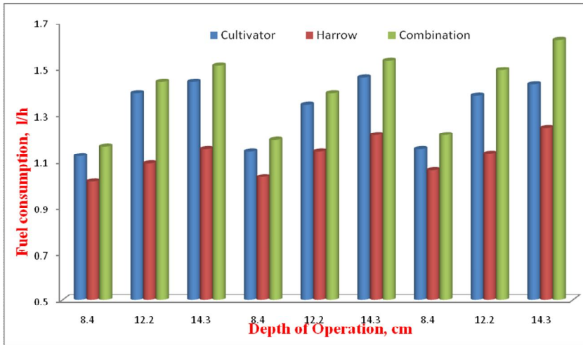
Fig.4: Effect of depth of operation on fuel consumption
