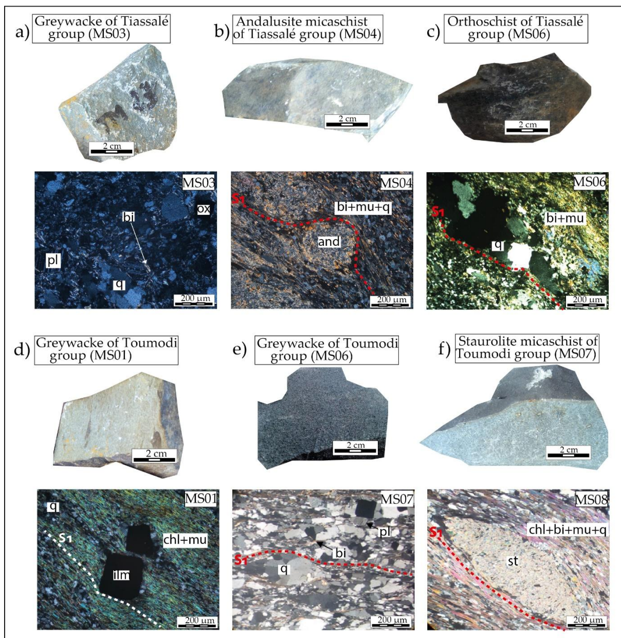
Fig. 4. Photographs and microphotographs of studied metasedimentary rocks of Comoé basin.
