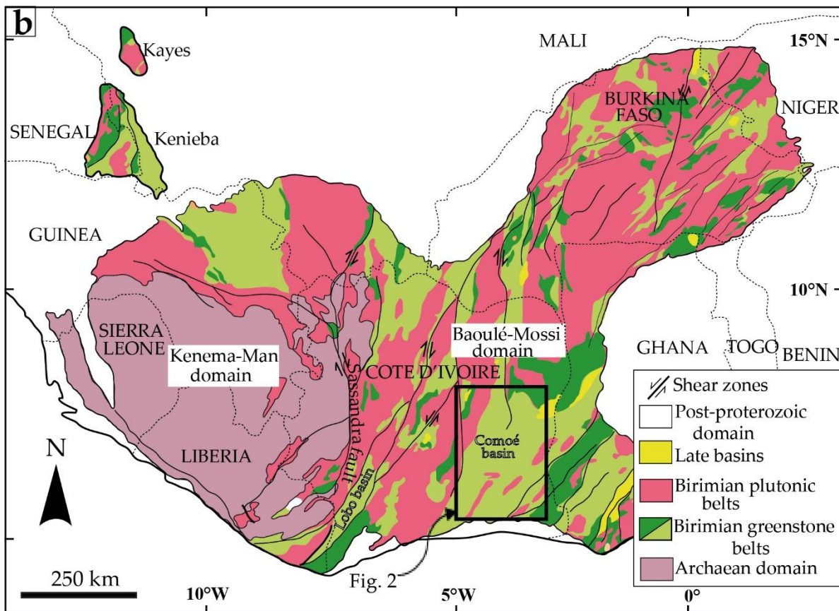
Fig. 1. Regional Geological maps.
