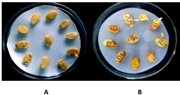
Figure 3: (a) un-treated soybean seeds (b) treated soybean seeds after incubation in the dark for 4 days. The treated soybean seeds induced glyceollin upon treatment with the bacterial alginate. The colour change witnessed was as a result of the presence of phytochemicals induction
