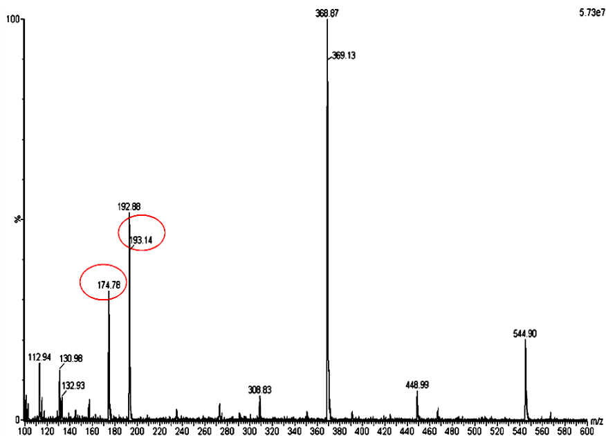
Figure 2: (ESI-MS) mass spectra of guluronic and mannuronic (G and M) fractions which were collected by preparative HPLC. The mobile phase used during the mass spectrometry analysis are (methanol / water = 1:1, v/v) which was delivered at a flow rate of 200 \mu l/min
